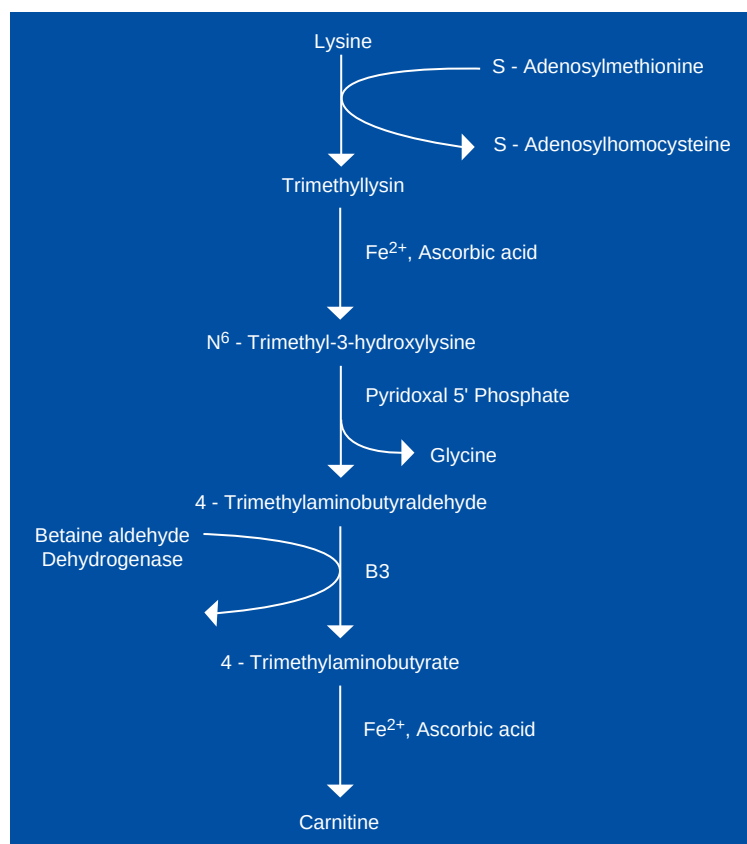
FIGURE 6. Carnitine synthesis
