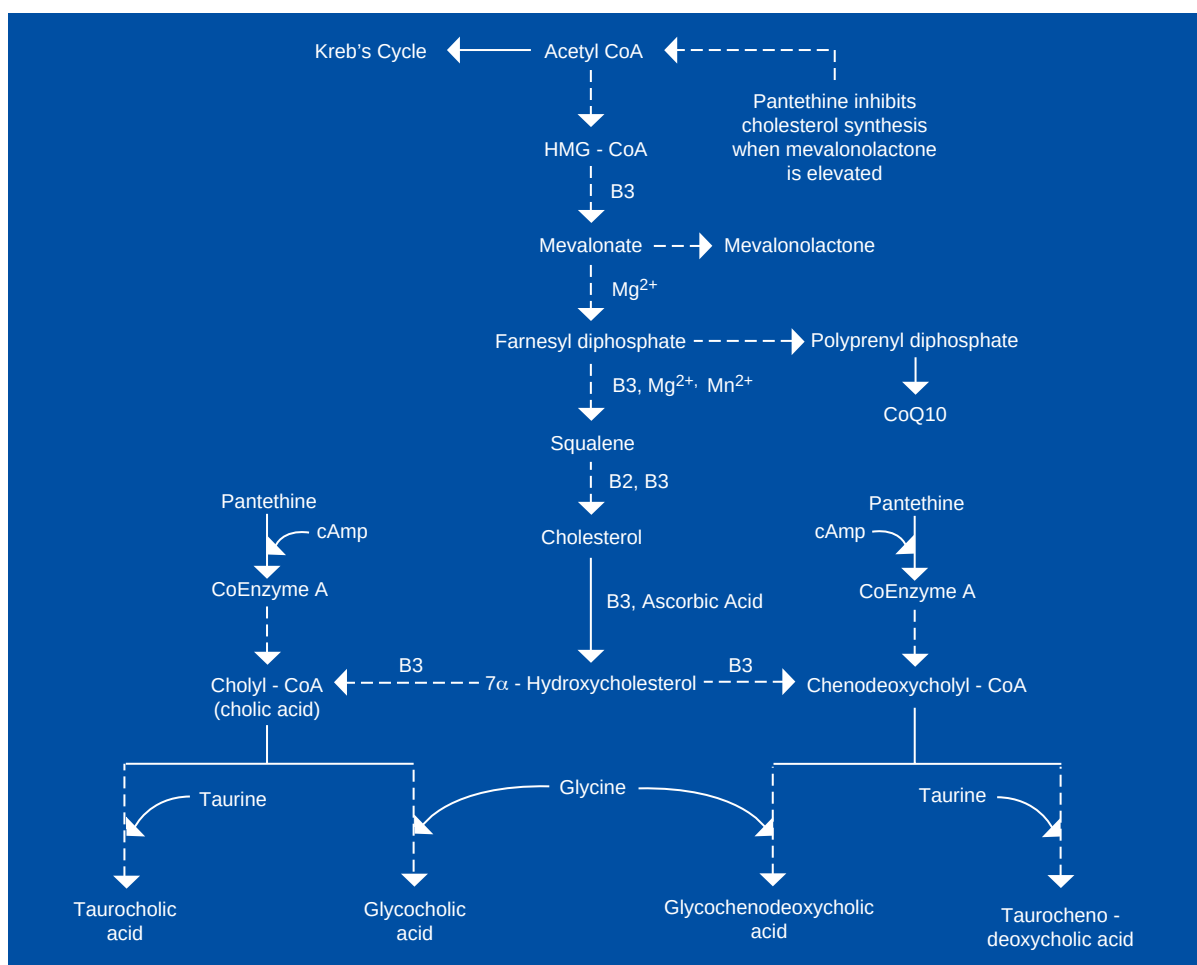
FIGURE 1. Cholesterol metabolism
